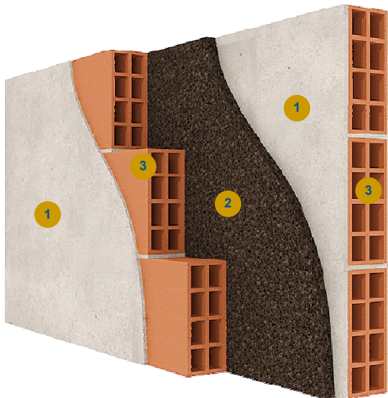
1 Roughcast 2 Expanded Cork Board - ICB 3 Double wall
